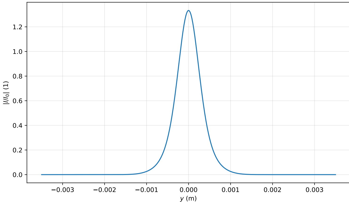
Intensity profile I(x=0, y, z=1.194)/I_0 , P_{in}=0.8P_{cr} , artificial time
